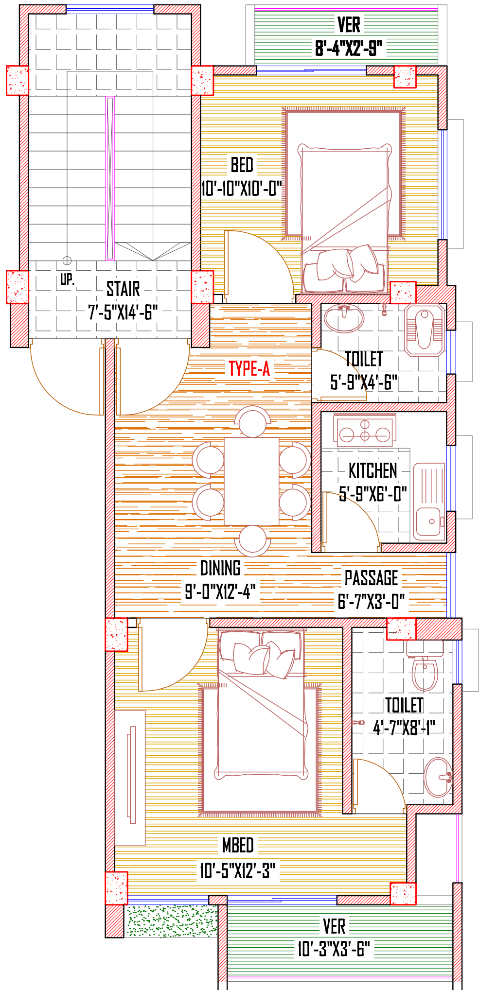
1ST - 5TH FLOOR PLAN TYPE-A 810 SFT.
