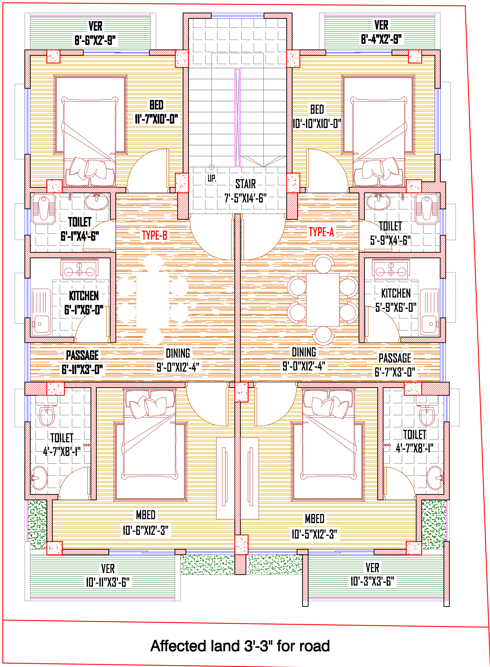
1ST - 5TH FLOOR PLAN
