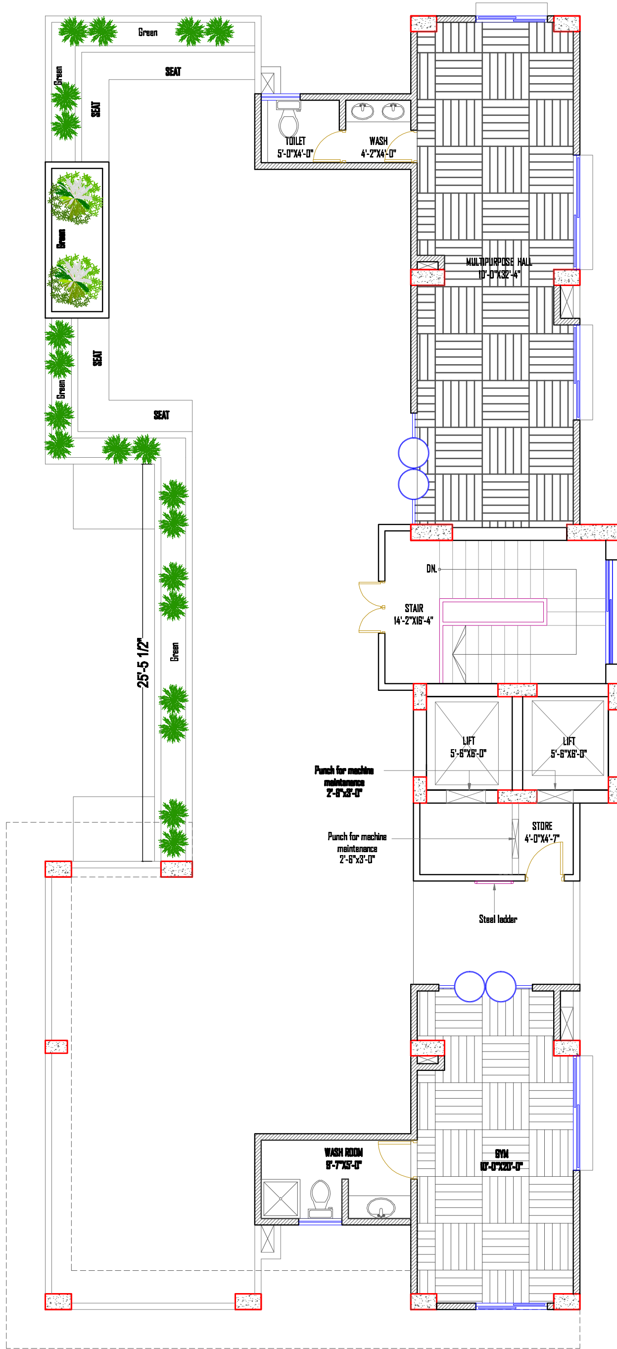
ROOF FLOOR PLAN-1
