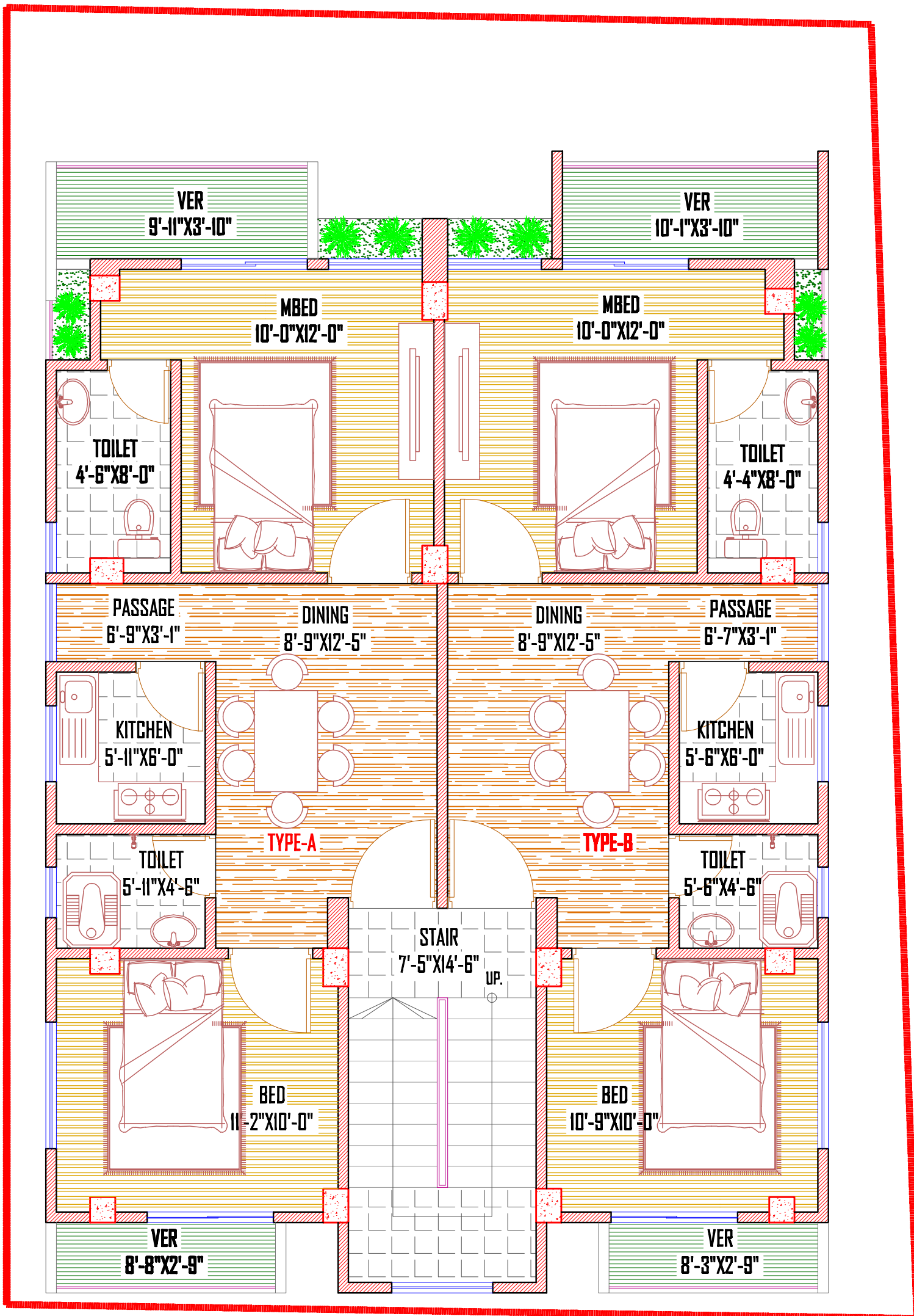
1ST -5TH FLOOR PLAN.
